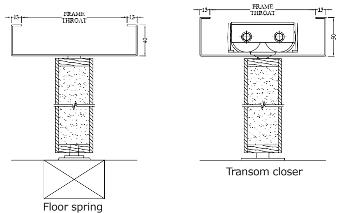
Typical head and floor section detail
